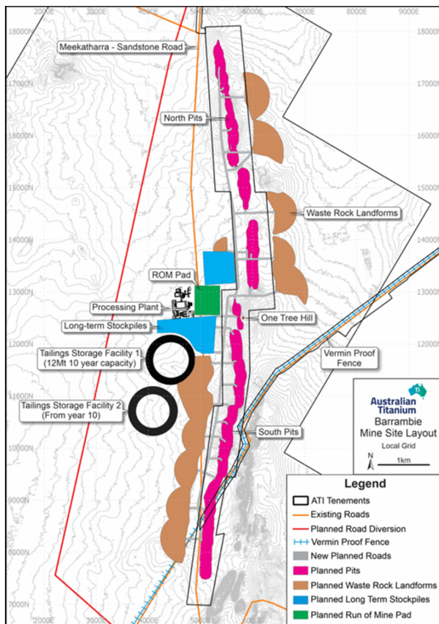
Figure 3: Overall Barrambie Mining Site Layout (local grid).
