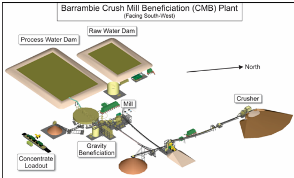
Figure 1: 3D Representation of Barrambie CMB Site
